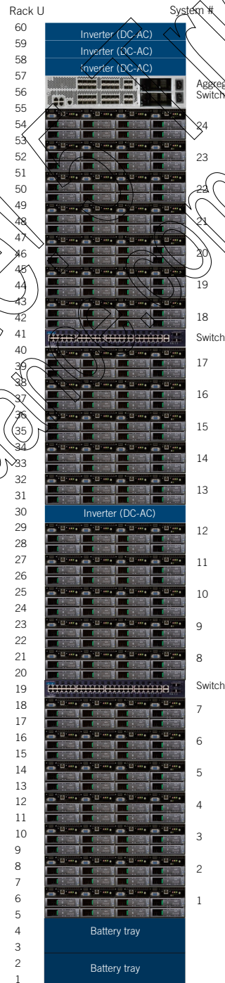
24 System rack layout
