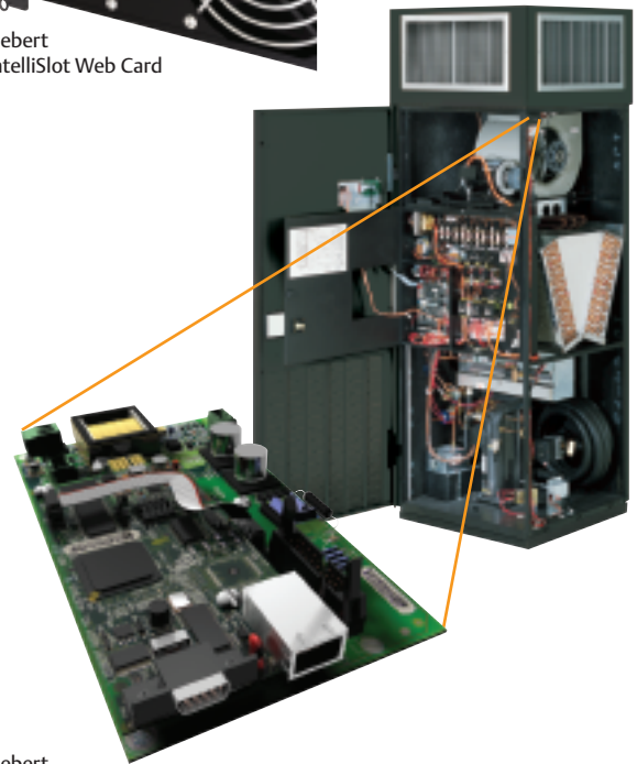
Liebert IntelliSlot Web/485 Card
